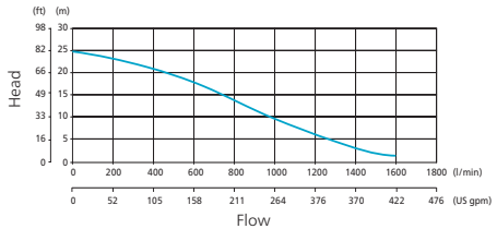
Performance curve
