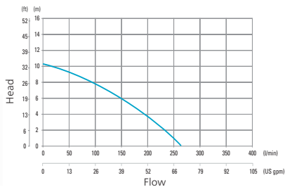
Performance curve
